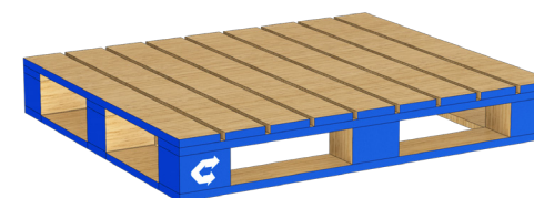
Chep houten UK pallet 1200 x 1000 mm
